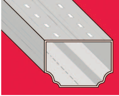
Double glazing profile H. 8
